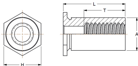
Partial Thread Version
